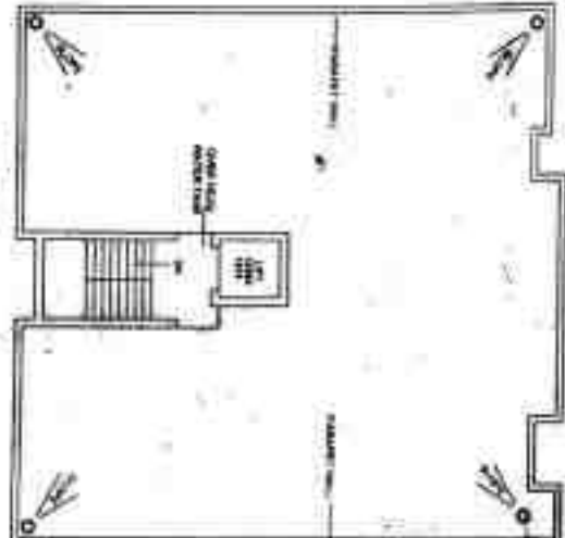
TERRACE FLOOR PLAN SCALE 1/8" = 1'-0"
